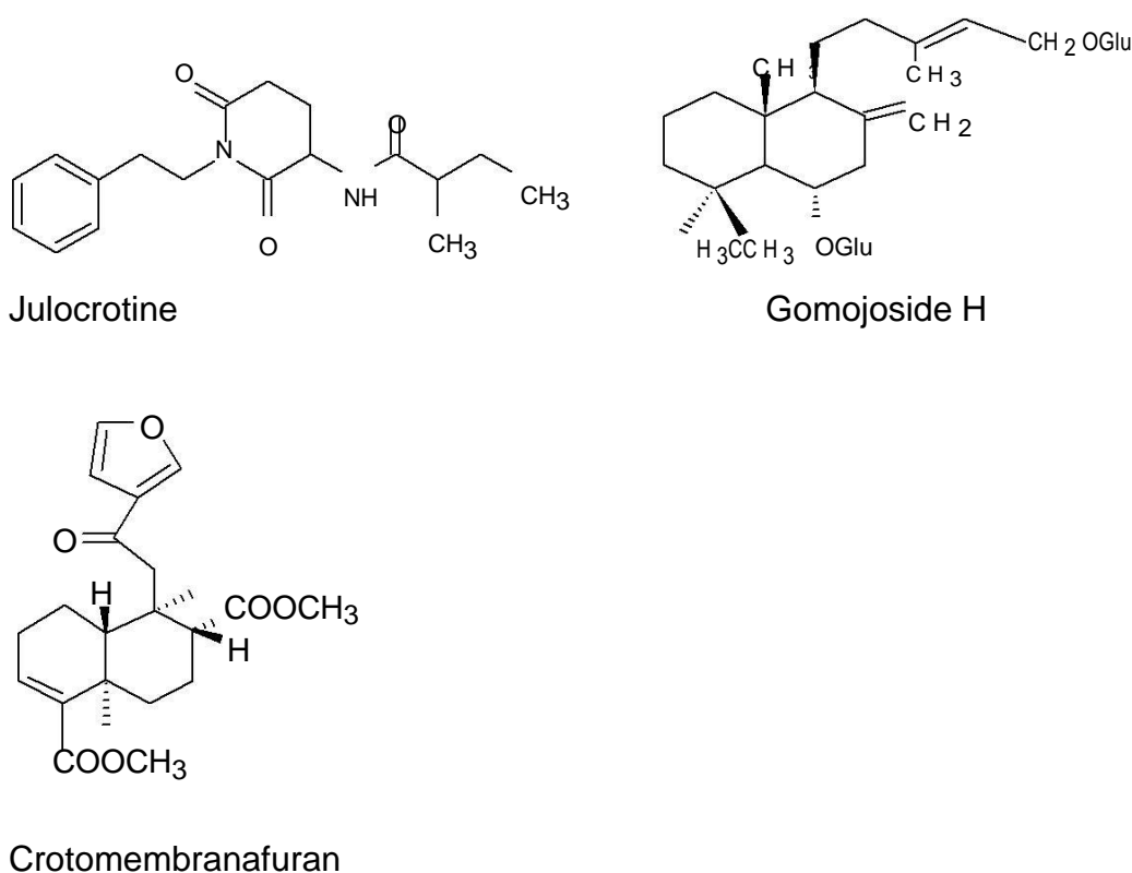
Figure 1. Some compounds obtained from C. membranaceus .
