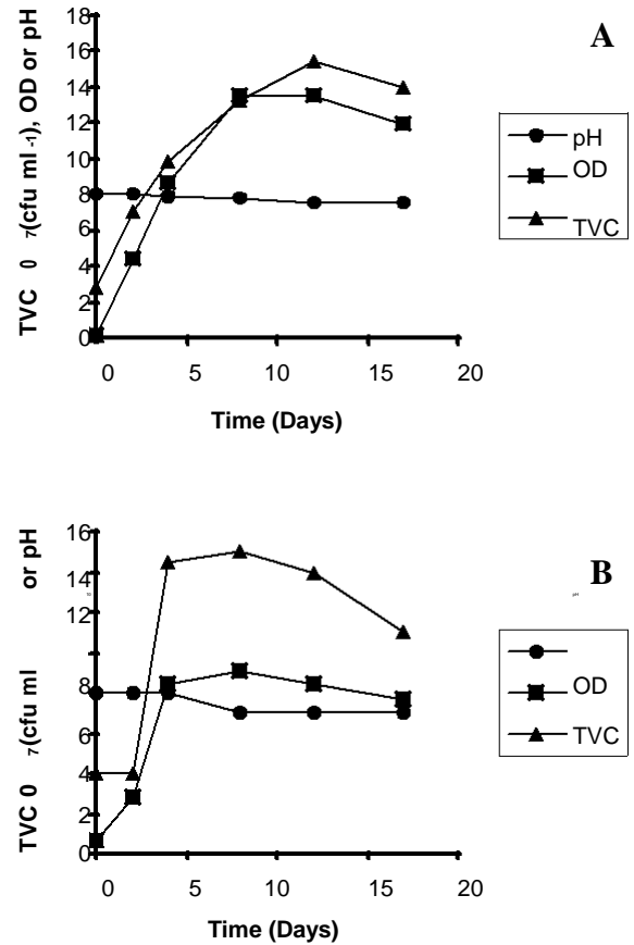
Figure 4. Growth profile of a mixed culture of Bacillus , Micrococcus , Proteus and Bacillus species. in mineral salt medium containing Bonny Light (A) and Bonny Medium (B) crude oil as sole source of carbon and energy.
