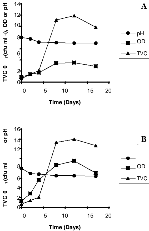
Figure 3. Growth profile of Micrococcus species in mineral salt medium containing Bonny Light (A) and Bonny Medium (B) crude oil as sole source of carbon and energy.
