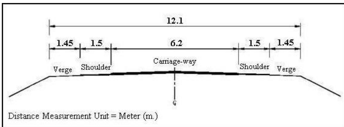
Figure 1: Standards of cross-sectional elements applicable for study road Source: Government of the People's Republic of Bangladesh, 2000
