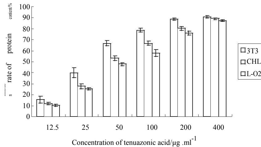
Figure 4. Effect of tenuazonic acid on total protein contents of the 3T3, CHL, and L-O2 mammalian cells exposed 72 h to tenuazonic acid at concentrations from 12.5 to 400 µg/ml. At the end of the treatments, total protein contents were measured by Lowry (1951) method.
