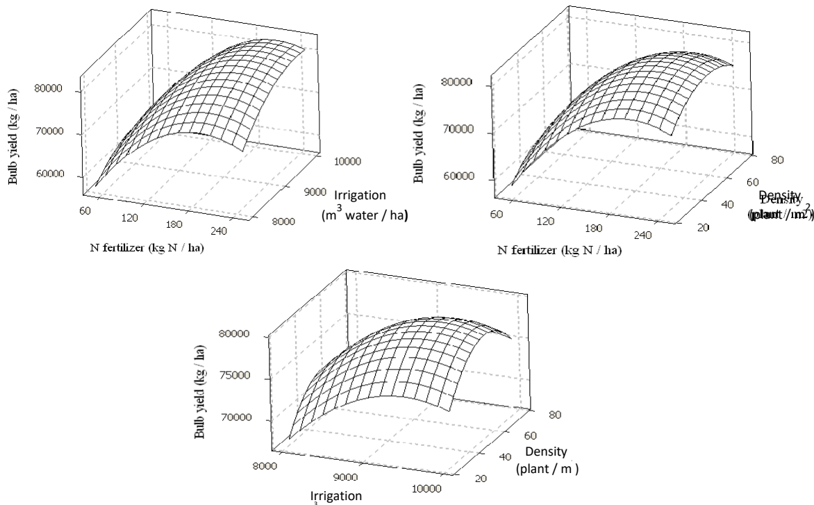
Figure 2. The bulb yield response to independent variables of N fertilizer, irrigation and density.
