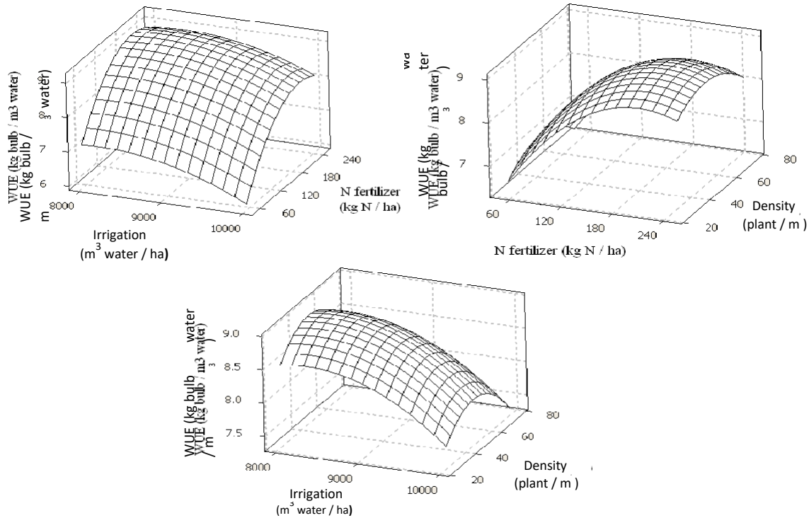
Figure 5. The WUE ( \text{kg bulb} / \text{m}^3 \text{ water} ) response to independent variables of N fertilizer, irrigation and density.
