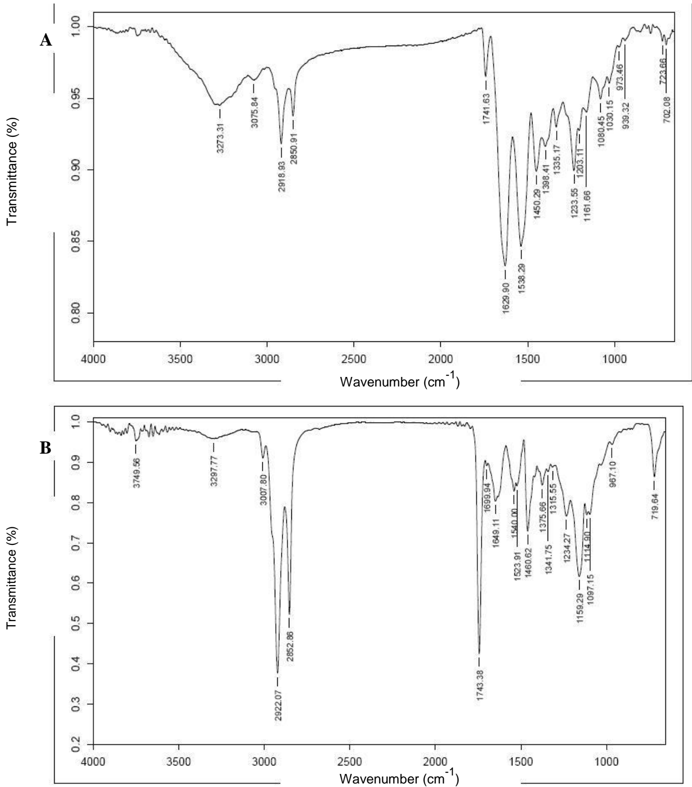
Figure 2. FTIR spectra of gelatin from skin of striped catfish (A) with no and (B) with bleaching.
