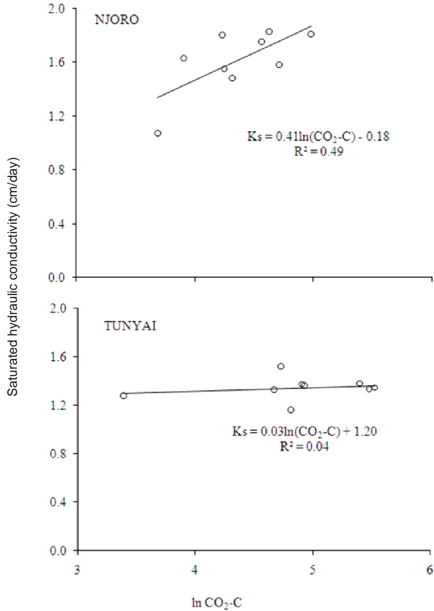
Figure 4. Saturated hydraulic conductivity (Ksat) as a function of CO 2 -C evolution for the soils from the two locations.
