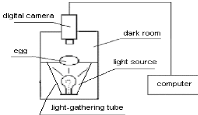
Figure 1. Machine vision imaging system.
