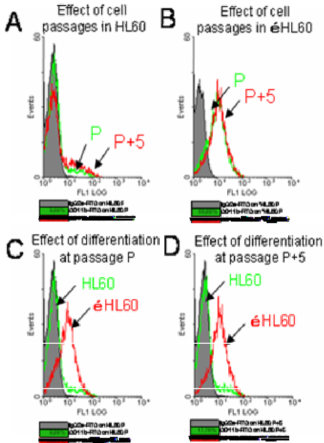
Figure 1. Flow cytometry analysis of CD11b surface expression expressed in percentage of positive cells: effect of cell passages (A and B) and effect of DMSO-differentiation (C and D) on CD11b surface expression on HL60 and HL60 at passage P and P+5. Graphs represent the number of cells (Events) as a function of fluorescence intensity (FL1 LOG). The gray areas show control fluorescence due to an unspecific antibody (IgG2a) for the studied cells. Results are percentages of CD11b-positive cells, measured with FITC-conjugated anti-CD11b antibodies at 488 nm. Representative experiment among at least 3 independent experiments.
