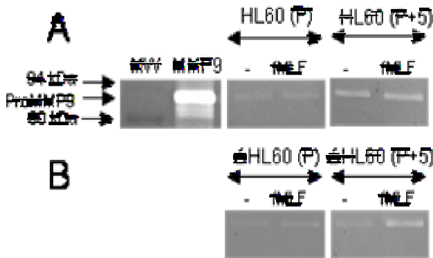
Figure 2. Zymographies: Effects of cell passaging on MMP9 zymographic activity in supernatants of HL60 (A) and HL60 (B), under basal or fMLF-stimulated conditions. MW: Molecular weight prestained SDS-Page standard broadrange markers, in kDa. MMP9: human recombinant control. Representative zymographies among at least 3 independent experiments.
