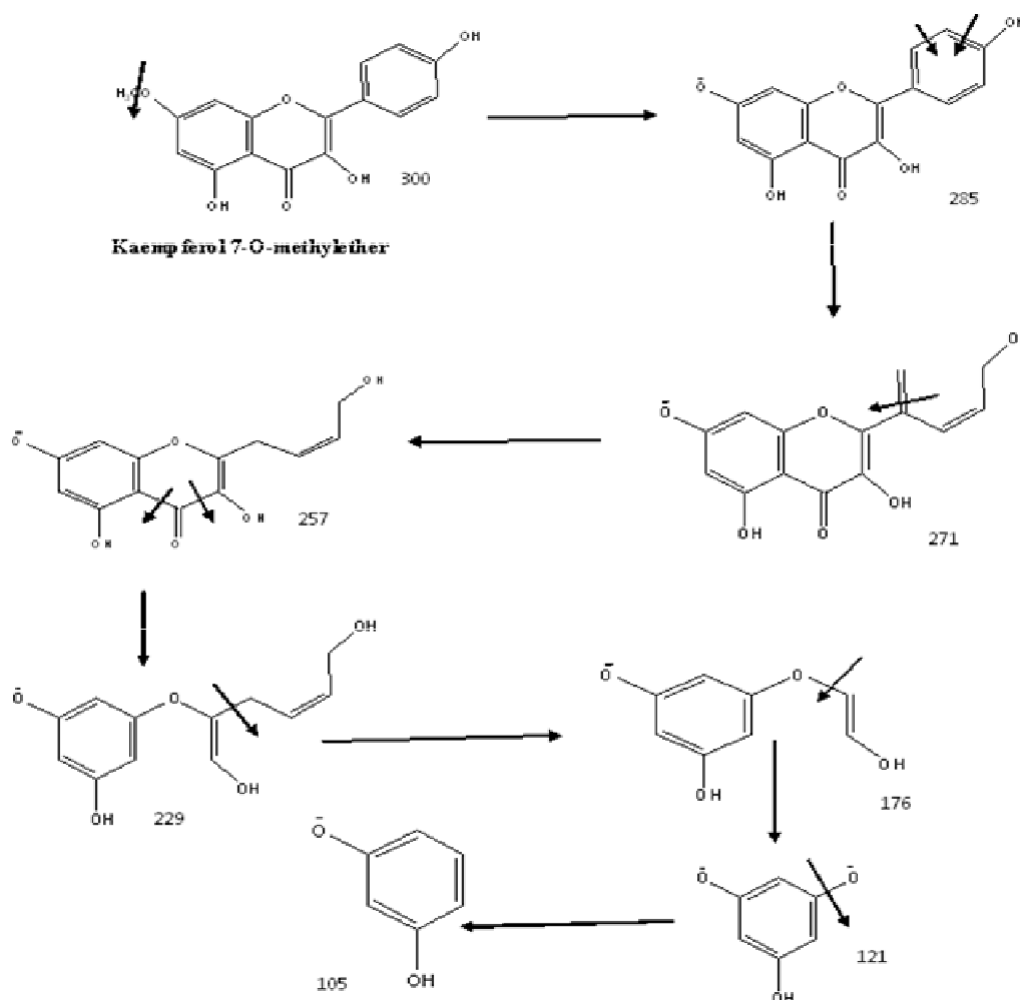
Figure 5. The fragmentation pattern of Kaempferol 7-O-methylether.
