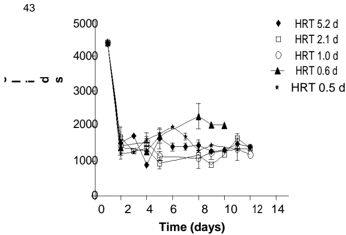
Figure 3. The total solids removal during anaerobic treatment of potato-processing wastewater at 37°C using a UASB reactor at various HRTs (n = 2).
