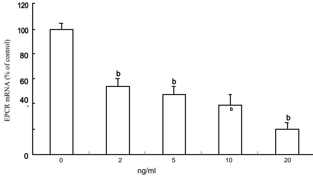
Figure 3. Effects of different concentrations of TNF- \alpha on EPCR expression. The mRNA level of EPCR was significantly decreased. A, p < 0.05 ; b, p < 0.01 , compare with the control (0 ng/ml).
