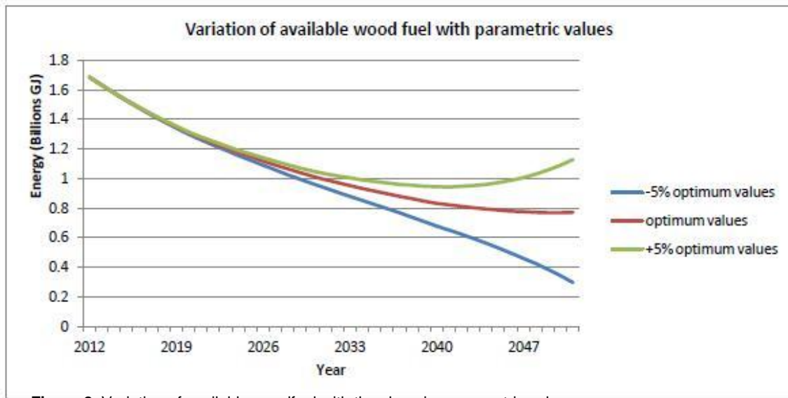
Figure 2. Variation of available woodfuel with the changing parametric values.
