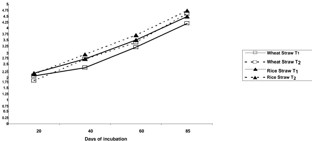
Figure 2. Mineralization of nitrogen from 15 N labeled crop residues under varying temperatures. T 1 and T 2 refer to 20 and 35°C, respectively.
