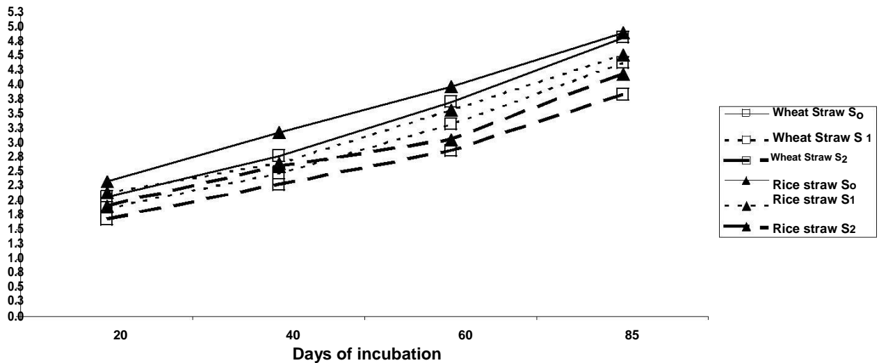
Figure 1. Mineralization of Nitrogen from 15 N labeled crop residues under varying clay content. S 0 , S 1 , S 2 refer to original soil, 75% original soil + 25% sand and 50% original soil + 50% sand respectively.
