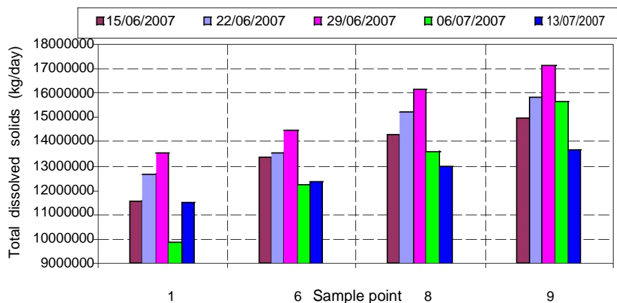
Figure 21. Variation of total dissolved solids in kg/day along the Lakhya River.
