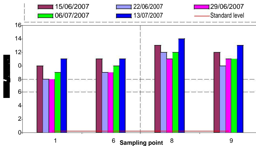
Figure 3. Variation of BOD 5 in mg/l along the Lakhya River.
