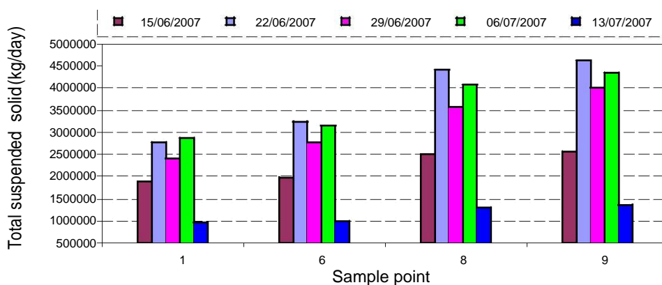
Figure 20. Variation of total suspended solids in kg/day along the Lakhya River.
