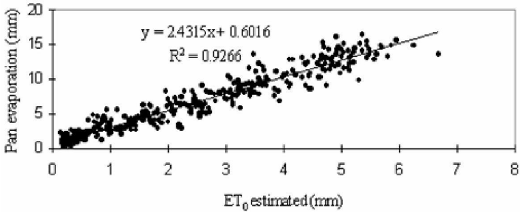
Figure 3. Comparison between the estimated ET_0 and pan evaporation at the experimental site in 2004.
