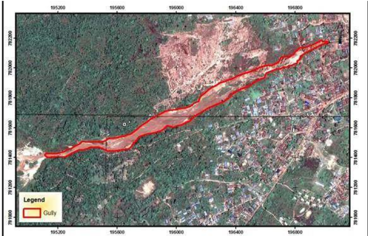
Figure 5. Satellite imagery (spot 7) showing the gully in 2012 (Source: Spot image).
