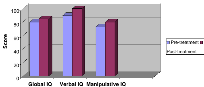
Figure 4. Changes of intelligence scores (before and after NF treatment).
