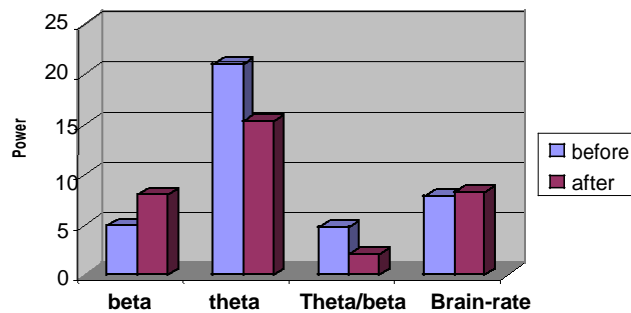
Figure 3. Changes of biofeedback parameters (before and after NF training).
