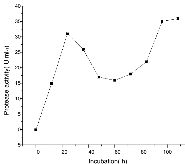
Figure 3. Protease Production pattern of Bacillus sp. K-30 at optimum pH and temperature.
