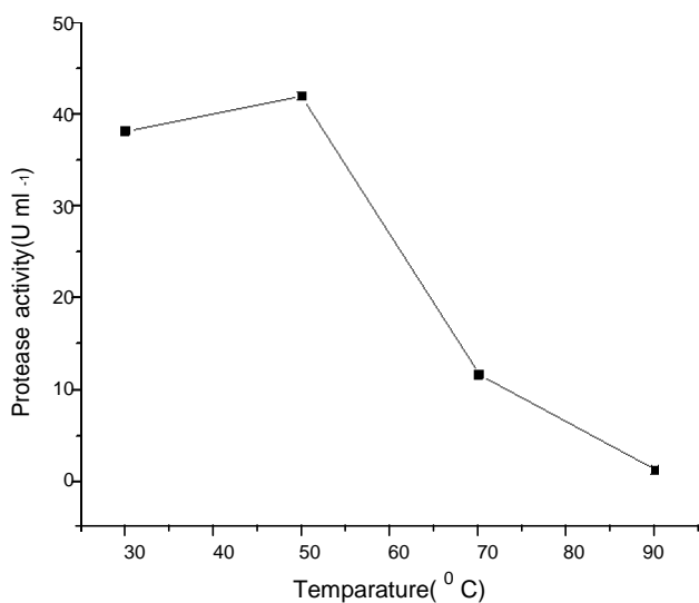
Figure 2. Production of protease by Bacillus sp. K-30 at different temperature using rice bran.
