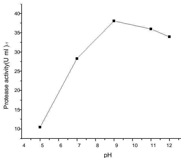
Figure 1. Production of protease by Bacillus sp. K-30 at different pH using rice bran.
