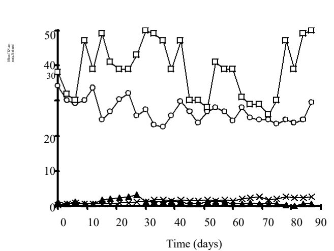
Figure 5. Effluent BOD, COD, TP and SS profiles of wetland system operated with soil sand ratio of 75:25, 50:50 and 25:75 at HRT of 0.75 day. BOD (●), COD (◇), SS (■), TP (△), TKN (□), ammonia (○), nitrite (●) and nitrate (x).
