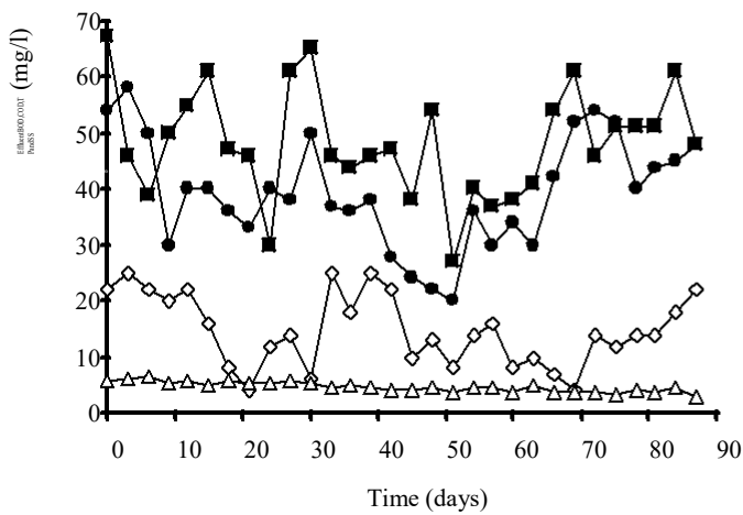
Figure 5. Effluent BOD, COD, TP and SS profiles of wetland system operated with soil sand ratio of 75:25, 50:50 and 25:75 at HRT of 0.75 day. BOD (●), COD (◇), SS (■), TP (△), TKN (□), ammonia (○), nitrite (●) and nitrate (x).
