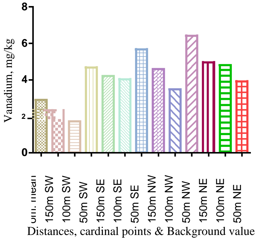
Figure 11. Concentration of vanadium based on distances, cardinal points and background value.
