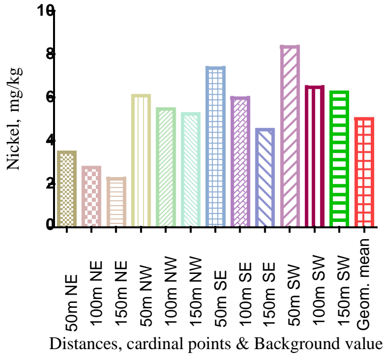
Figure 10. Concentration of nickel based on distances, cardinal points and background value.
