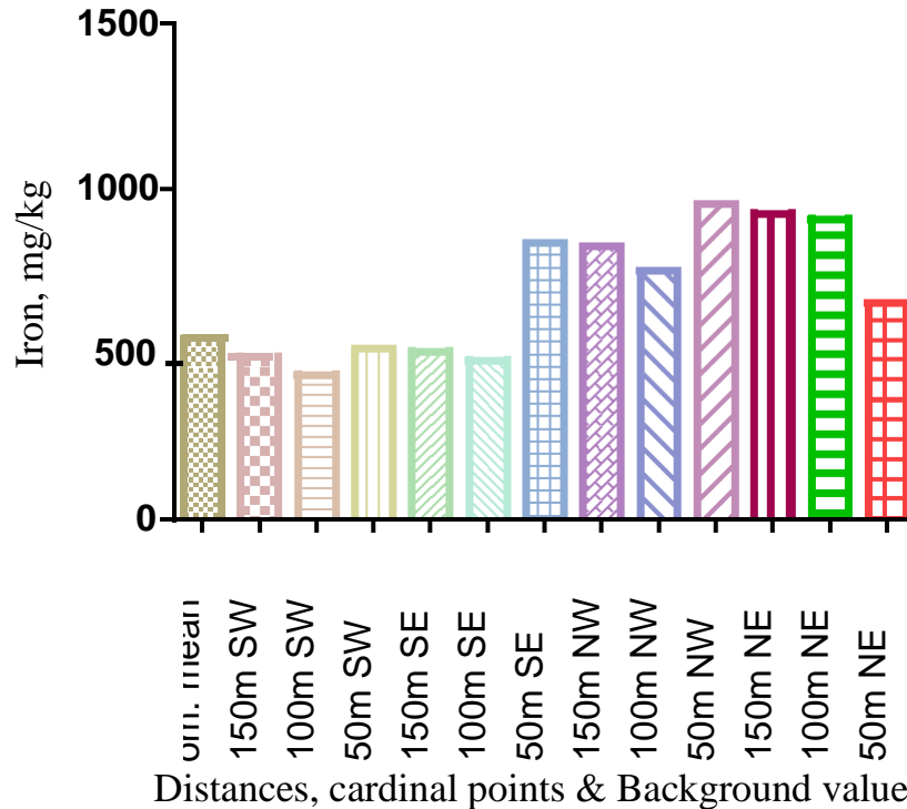
Figure 3. Concentration of iron based on distances, cardinal points and background value.
