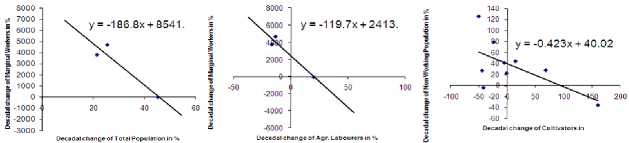
Figure 4. Significant negative relationship found from correlation co-efficient matrix.
