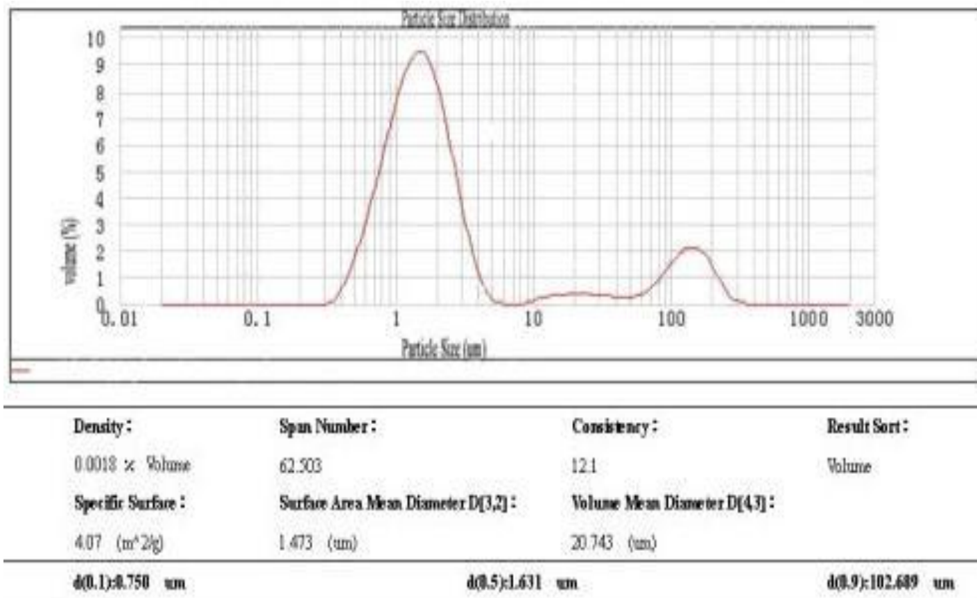
Figure 3. Particle size and distribution in percentage of volume. D[4, 3] is the mean diameter in volume whereas D [3, 2] is the mean diameter in surface called “Sauter diameter”; D(v, 0.5) is the size for which 50% of the sample particles has a lower size and 50% has a upper size; D (v, 0.1) is the size for which 10% of the sample particles has a lower size and D (v, 0.9) is the particle size for which 90% of the sample particles has a lower size. The particle size distribution width is characterized by the relation: [D(0.9) - D(0.1)]/D(0.5) which defines the span number.
