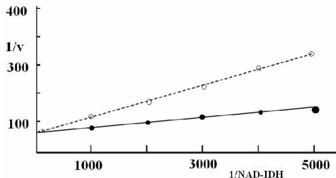
Figure 3. The effect on NAD-IDH in the presence (○) or absence (●) of ATP. The incubation mixture is as described under methods. NAD concentrations are varied while ATP concentration is fixed.
