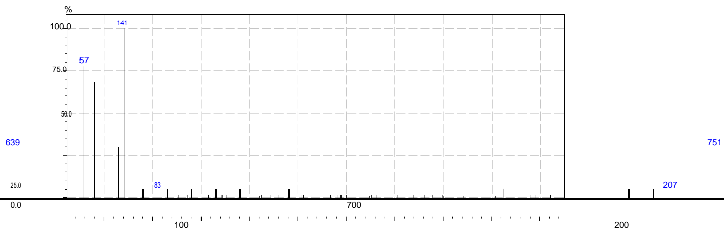
b. Anthracene [Retention time (RT) 9.670, m/z identification ion-178]
