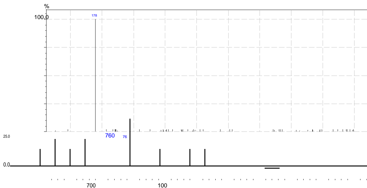
b. Anthracene [Retention time (RT) 9.670, m/z identification ion-178]
