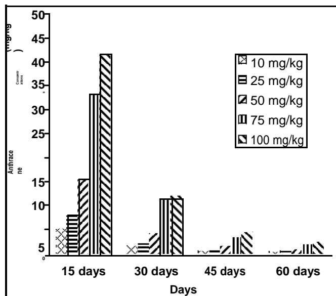
Figure 1. Concentration of anthracene found during the phytoremediation of anthracene contaminated soil using ryegrass.
