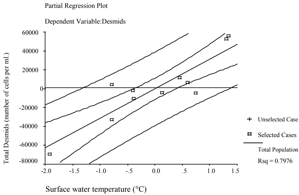
Figure 3a, b, c, d. Partial regression plots showing the relationship between the population of Desmids, Transparency, Salinity, Bottom Water dissolved Oxygen and Surface Water Temperature within the period of study.
