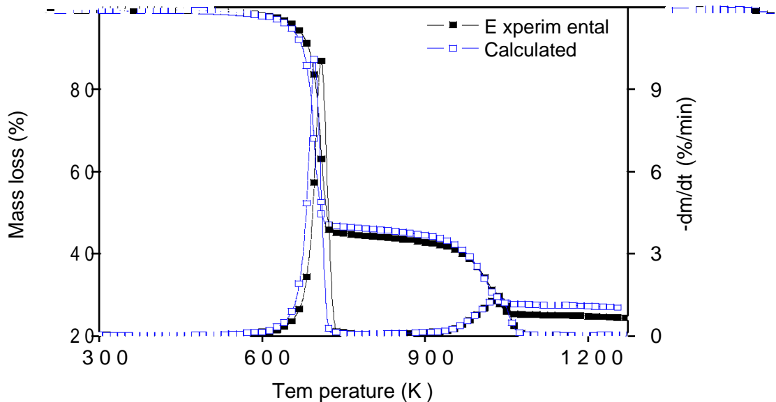
Figure 4. Comparison between experimental and calculated TG/DTG values for the oil shale/polystyrene mixture at 10 \text{ K min}^{-1} .
