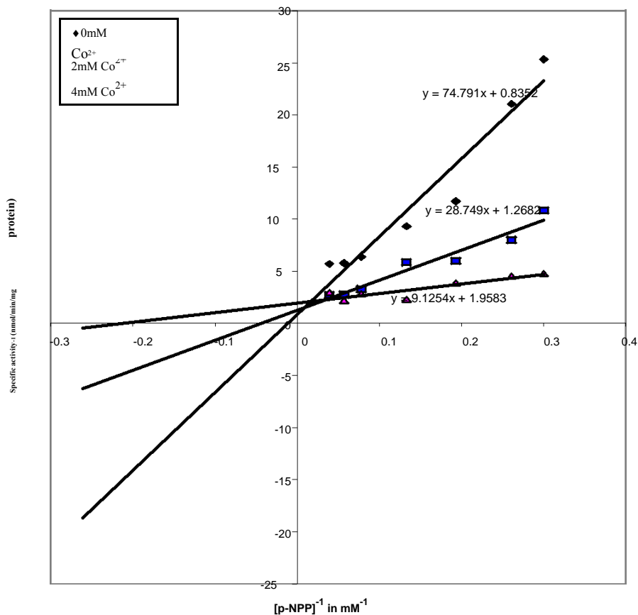
Figure 4. Double-reciprocal plot showing effect of \text{Co}^{2+} on rate of ALP-catalyzed hydrolysis of p-NPP.
