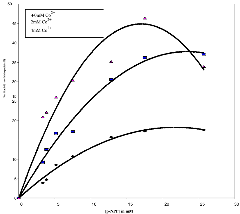
Figure 3. Michaelis-Menten's curve showing effect of \text{Co}^{2+} on rate of ALP-catalyzed hydrolysis of p-NPP.
