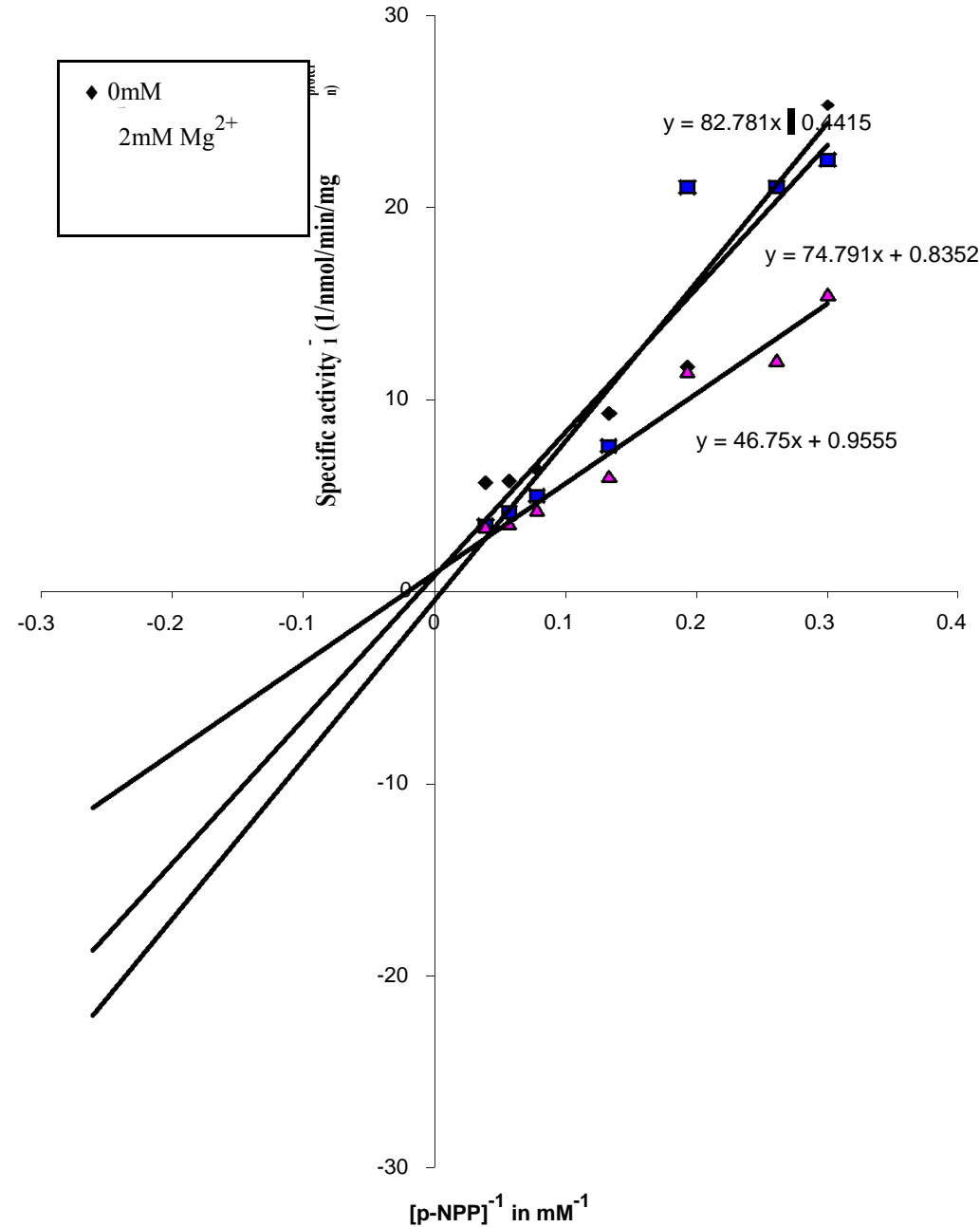
Figure 2. Double-reciprocal plot showing the effect of Mg^{2+} on rate of ALP-catalyzed hydrolysis of p-NPP.
