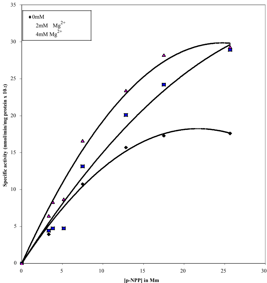
Figure 1. Michaelis-Menten's curve showing the effect of Mg^{2+} on rate of ALP-catalyzed hydrolysis of p-NPP
