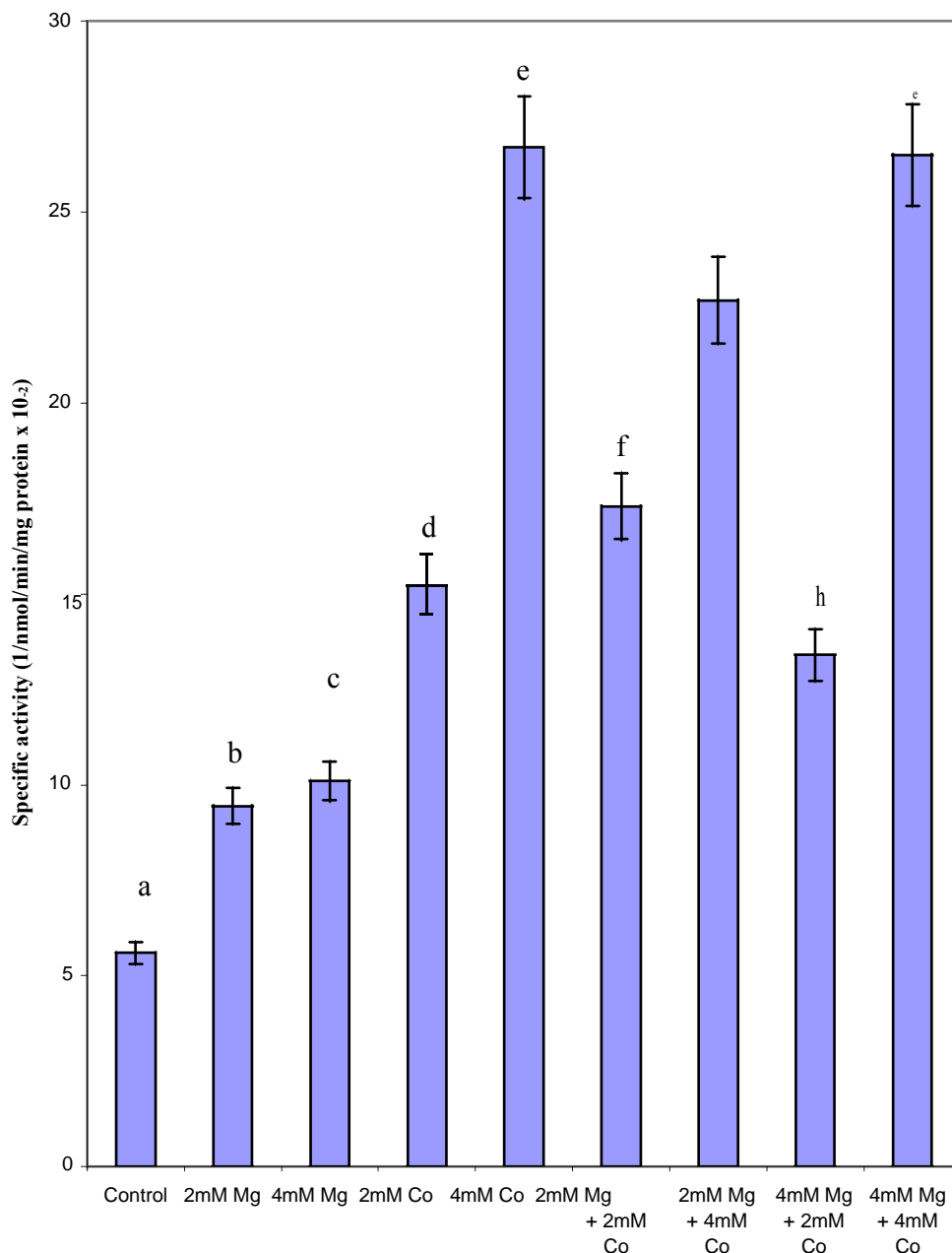
Figure 5. Bar-chart representation showing effect if interaction of Mg^{2+} and Co^{2+} ions on ALP activity at 5.17 mM p-NPP. Each value is an average of 3 determinations \pm SEM. Values are significant different in comparison with a, b, c, d, f, g and h at P < 0.05 .
